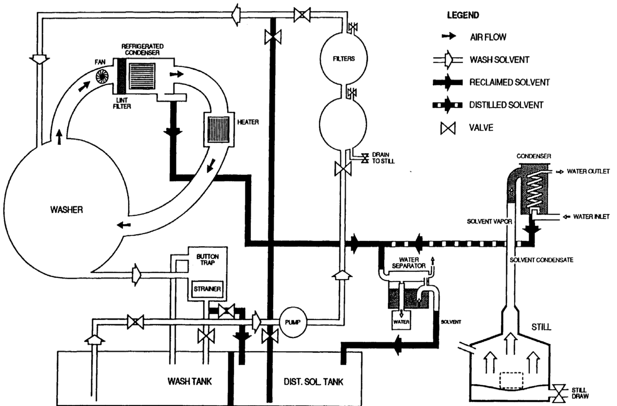
Operational Diagram of a Typical Dry Cleaning Machine
